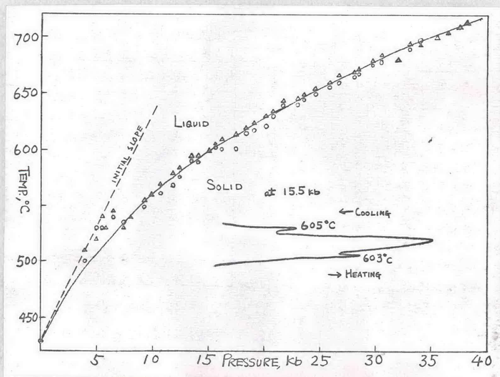
Fig. 5 Melting curves of AgCl ( \circ ..heating \Delta ..cooling)
